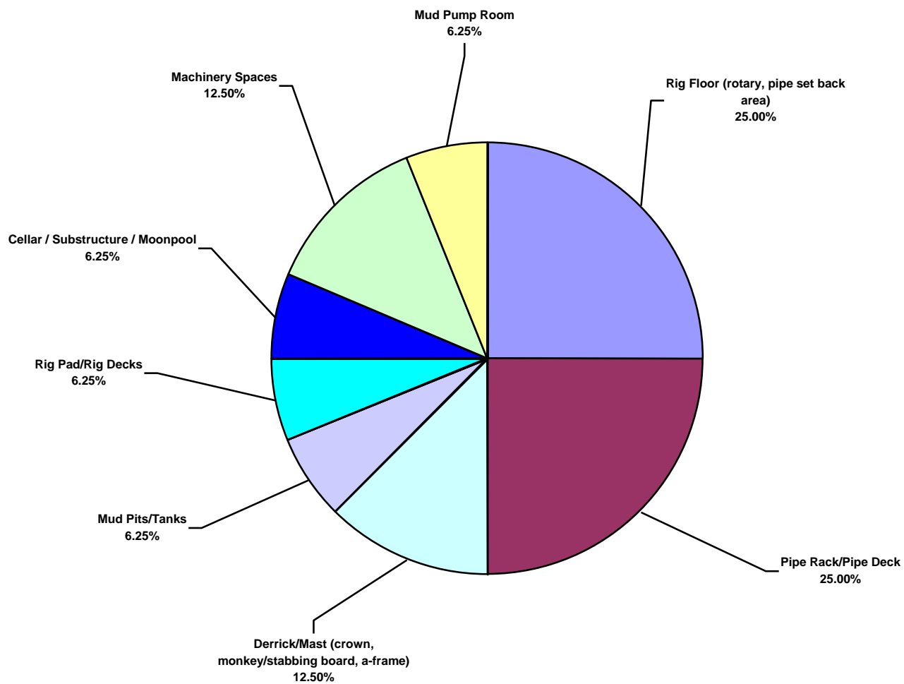
European Land Total Lost Time Incidents by Location (Chart 13) Based on 16 Incidents
