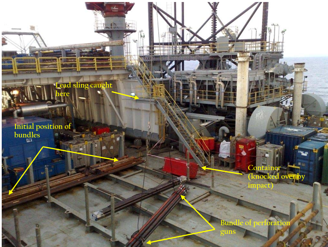
Overhead View of Main Deck, showing location of items related to the incident.
